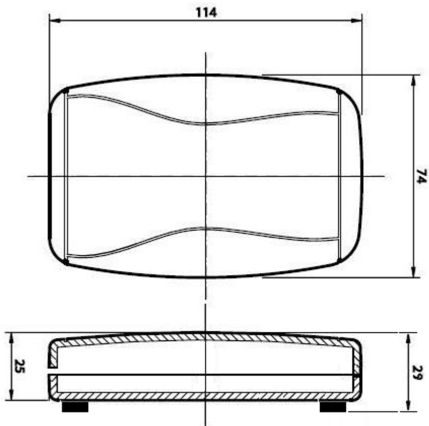
MT650 Desktop enclosure
